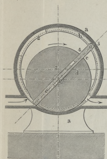
Fig. 5. Beale. Gaspumpe.
