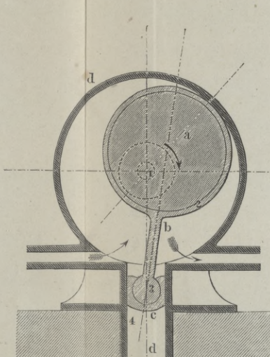
Fig. 4. Pattison, Pumpe.
