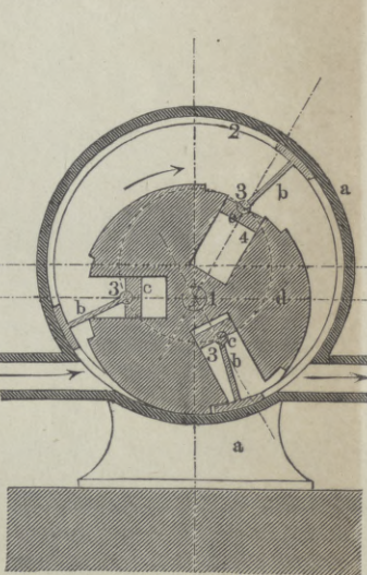
Fig. 18. Fletcher. Dpfm.
