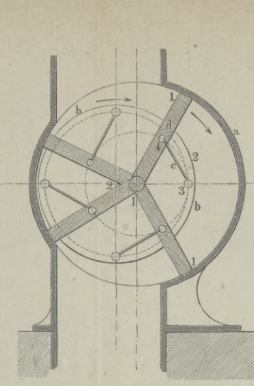
Fig. 13. Heppel. Pumpe.
