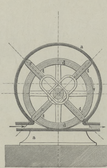
Fig. 6. Woodcock. Dpfm.
