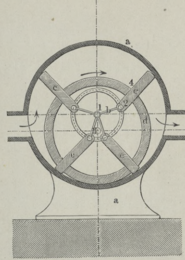
Fig. 3. Emery. Pumpe.
