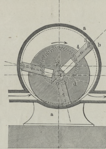
Fig. 6. Davies. Dpfm.
