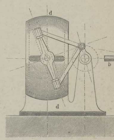
Fig. 3. Davies. Pumpe.
