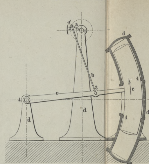
Fig. 9. Degrand. Dpfm.
