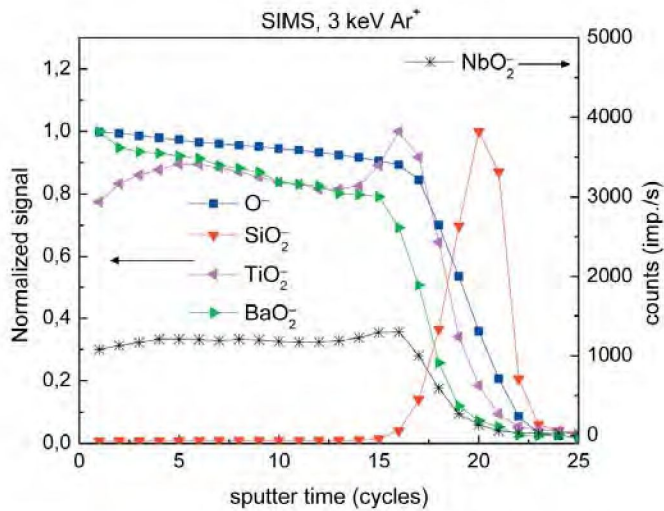
Fig. 2. SIMS profile of RF PS deposited BT film. Fig. 2. Profil SIMS warstwy BT.
