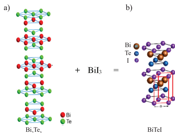
Fig. 3. The BiTeI compound structure, a) symmetrical unit cell (quintuple layers) of a \text{Bi}_2\text{Te}_3 topological insulator, b) asymmetrical unit cell with inversion of a BiTeI insulator with the dimensions indicated. Lattice parameters of BiTeI compound in the hexagonal plane a , along the growth axis - c are: a = 4.34 \text{ \AA} and c = 6.854 \text{ \AA} (according to Ishizaka et al. [5]).
