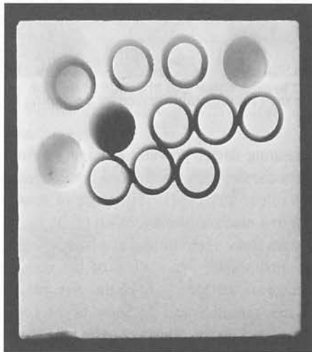
Fig. 6. Micro-cores in a marble sample. Lateral dimension of the specimen are 50 mm x 50 mm.
