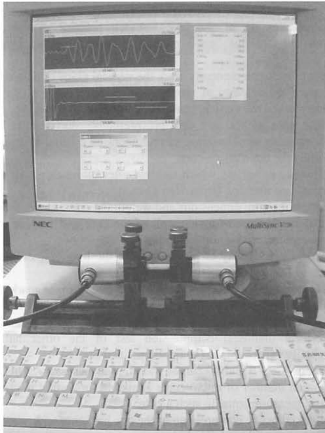
Fig. 7. Measurement of longitudinal wave in a microcore of Cervaiolle Marble (collaboration P. Gutkiewicz).
