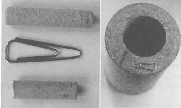
Fig. 1. Micro-cores taken out of sandstone and brick and a rock core from a mine.
