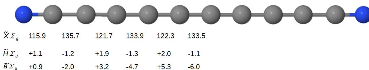
Figure 39. C 10 N 2 geometry in the ground and selected excited states, as derived at the B3PW91/aug-cc-pVTZ level of theory [192]. Distances in pm. Excited electronic state entries listed as relative to those of the ground state. D_{\infty h} symmetry was assumed.
