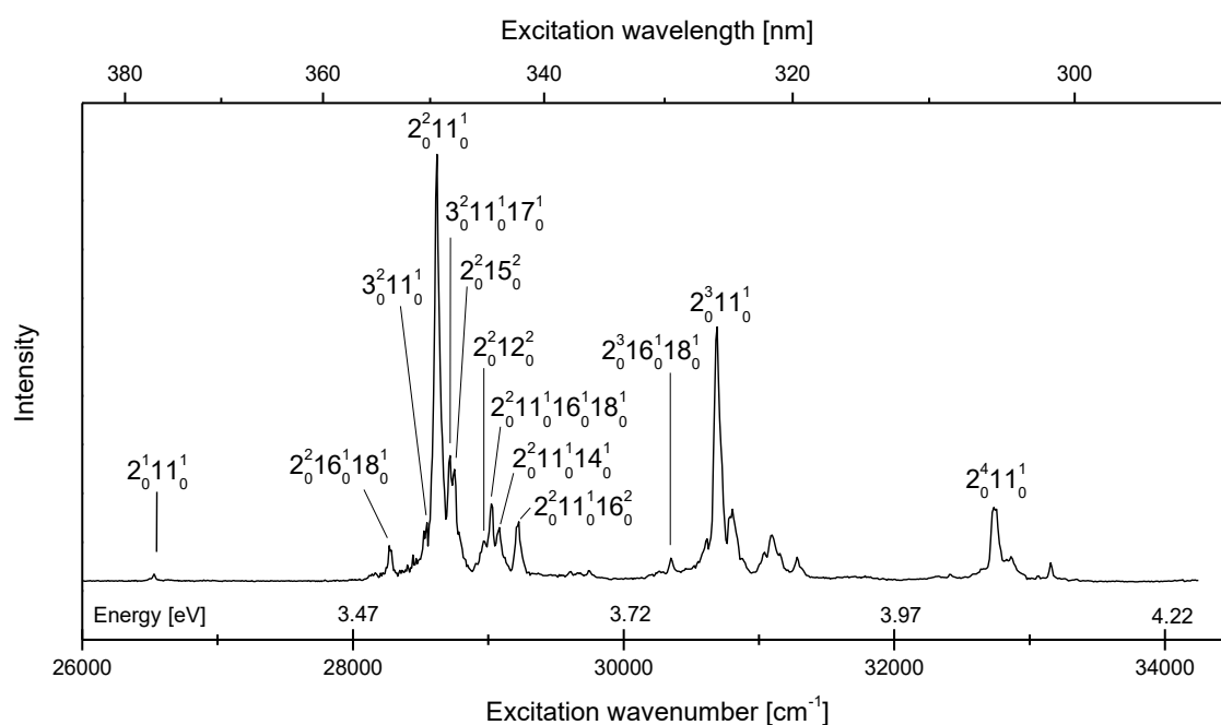
Figure 37. \tilde{B}^1\Delta - \tilde{X}^1\Sigma^+ system detected in the phosphorescence excitation spectrum of \text{HC}_9\text{N} , coming from a previously photolysed ( 193\text{ nm} ) \text{Kr}/\text{C}_4\text{H}_2/\text{HC}_5\text{N} ( 1000/1/1 ) matrix. Detection centred at the most intense phosphorescence band ( 17\,300\text{ cm}^{-1} , 2.14\text{ eV} ). The applied laser intensity correction may distort the phosphorescence intensity pattern.
