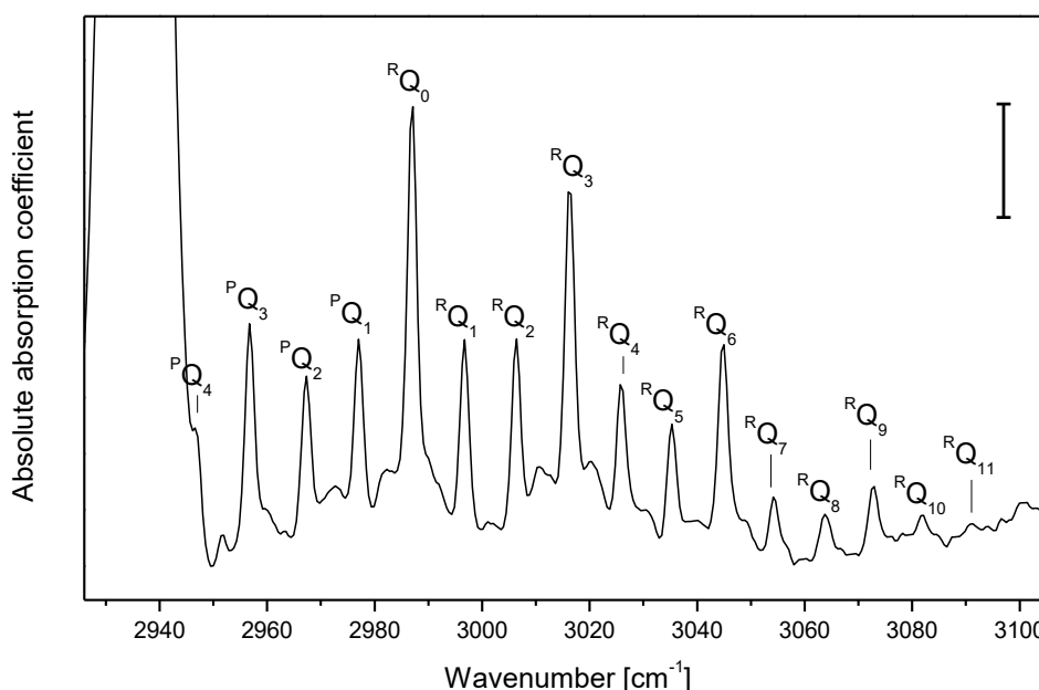
Figure 15. The rovibrational structure of \nu_9 in the IR absorption spectrum of gaseous \text{CH}_3\text{C}_5\text{N} . The strong leftmost feature is due to \nu_{11} . Vertical bar corresponds to the absolute absorption coefficient change equal to 0.1\text{ cm}^{-1}\text{ atm}^{-1} , as calculated for 294 K, at base e .
