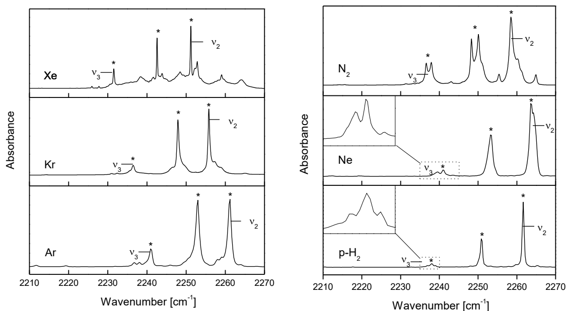
Figure 13. The \nu_2, \nu_3 region in IR absorption spectra of \text{CH}_3\text{C}_5\text{N} isolated in various cryogenic hosts. Asterisks mark three bands presumably coupled by an anharmonic interaction (the middle one likely comes from \nu_5 + \nu_7 ). Absorbance scales differ to increase the visibility of the detected spectral features.
