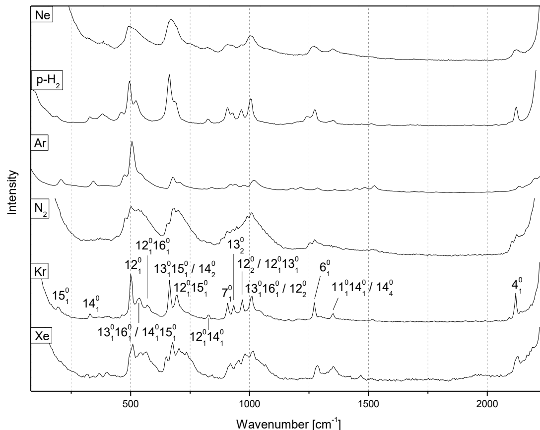
Figure 20. \text{CH}_3\text{C}_5\text{N} phosphorescence in various matrices. Spectra aligned with respect to the vibrationless \tilde{a}-\tilde{X} origins, arbitrarily set to 0\text{ cm}^{-1} . Assignments refer to Kr matrix values.
