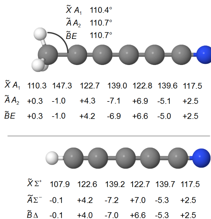
Figure 9. Geometry of \text{CH}_3\text{C}_5\text{N} and \text{HC}_5\text{N} in the ground and first excited singlet electronic states, as derived with CCSD/cc-pVDZ (ground state) or EOM-CCSD/ccpVDZ (excited states) levels of theory (adapted from [197]).
