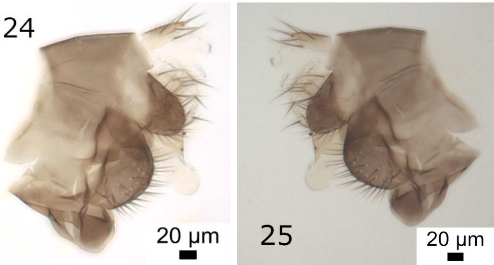
Figs 24–25. Tendcornphora microgenitalis Disney, male: 24 – left face of hypopygium; 25 – right face of hypopygium
