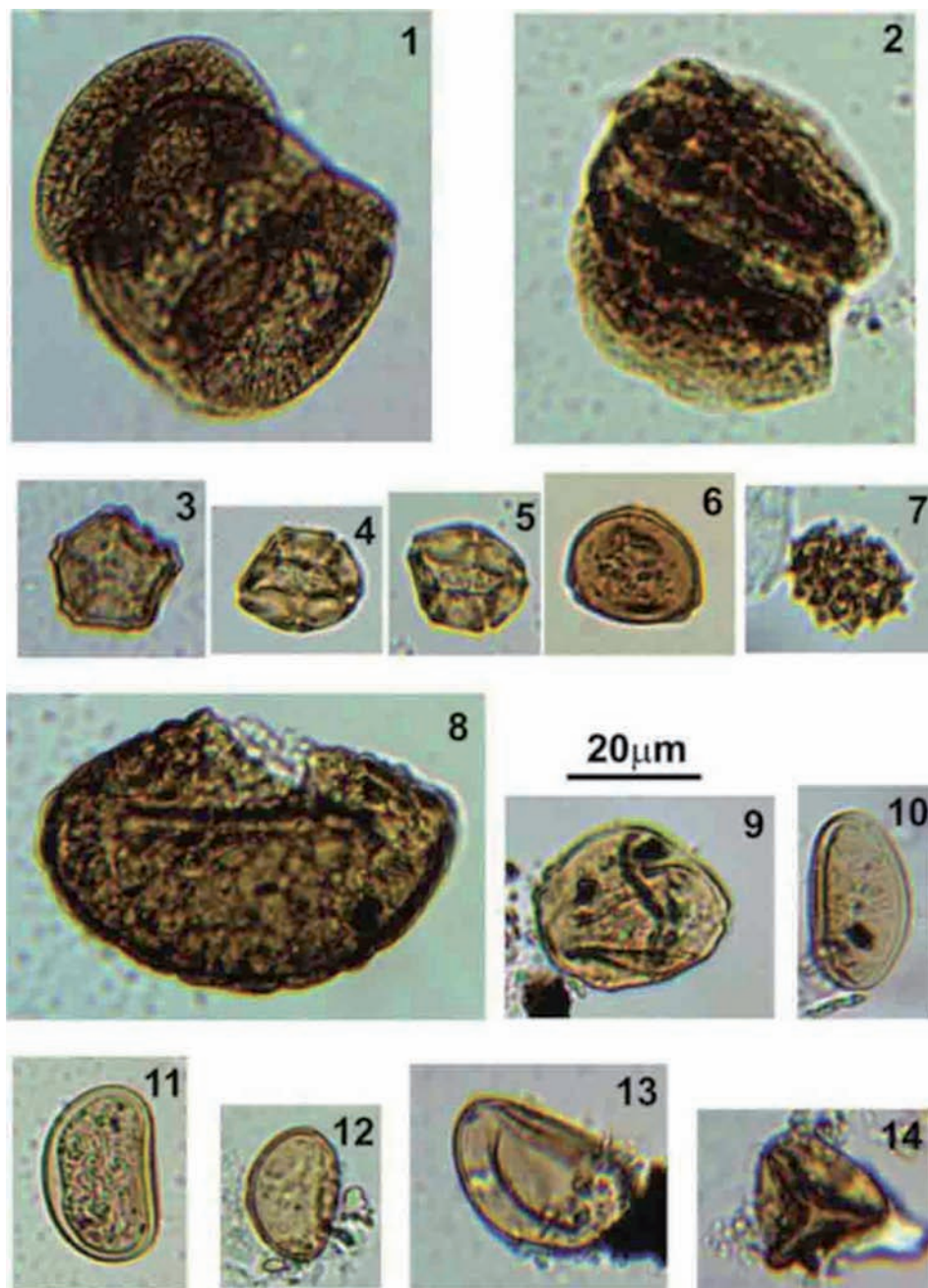
Fig. 6. Pollen grains of the plants and spores of ferns identified in the second sample: 1-2 – Pinus (Pine), 3-5 – Alnus (Alder-tree), 6 – Corylus (Hazel), 7 – Aster (Aster), 8, 10-14 – Polyodiaceae , 9 – Carpinus (Hornbeam) (photo by M. Chichinadze)
