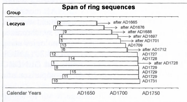
Fig. 1. Dating structural parts of the rafter framing from the church at Łęczyca.
