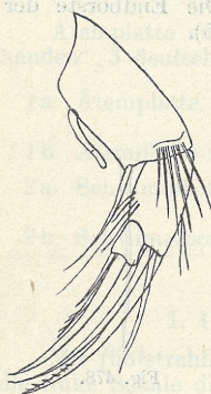
Fig. 479. 2. Antenne von Paracypridopsis variegata Br. Norm.
