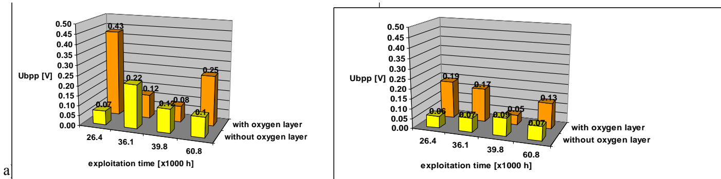
Fig. 1. The Barkhausen noise results coming from trailing edge a), leading edge; b) of turbine blades
