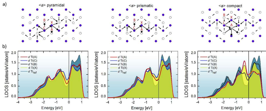
Fig. 1. Detailed structures of selected <a> type screw dislocation cores (a) and local density of states plots determined for X, C, B and A atomic position (b) [8]
