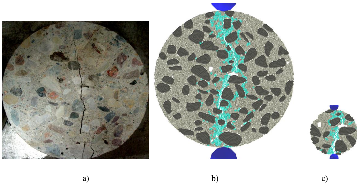
Figure 1: Fracture in concrete specimen in splitting tensile test in a) experiment and DEM calculations with 2 different specimen diameters: b) D=0.15 m and c) D=0.05 m (black colour indicates aggregates, grey colour represents cement matrix, white colour shows macro-pores, cyan colour denotes area with broken contacts and blue colour shows supports)
