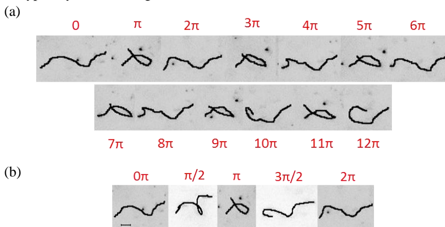
Figure 4.20. Characteristic bent-like configurations of long hydrogel nanofilaments ( \underline{L} = 500 ) at different time points over the course of an experiment (a) and during one oscillatory cycle (b).
