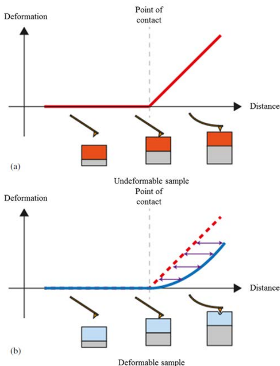
Figure 4.2. Scheme of force-distance evaluation for AFM indentation of a hard sample (a) and a soft sample (b). The curve of indentation can be obtained by subtracting one curve from the other, as indicated by the violet arrows [79].
