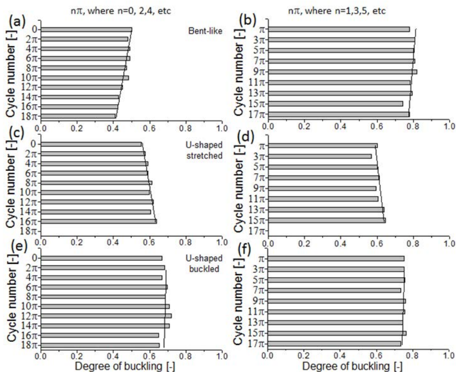
Figure 4.23. Time-dependent changes in the degree of buckling for bent-like (a, b), U-shaped stretched (c, d) and U-shaped buckled (e, f) hydrogel nanofilaments at each individual forward (left column) and reverse (right column) oscillatory cycle. Nanofilaments were subjected to a maximum of 9-10 consecutive oscillatory runs. Solid lines mark the data trend.
