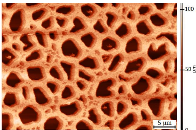
Figure 3.7. AFM surface topography of 100 nm polystyrene particles immersed in Triton X-100/Methanol (1:1); particles concentration 1:100, poured onto the silicon substrate.
