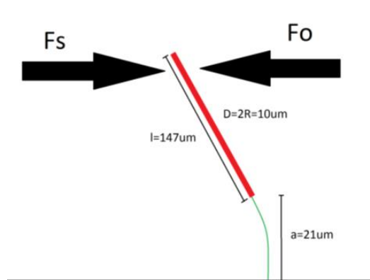
Figure 4.3. Scheme presenting forces acting on the deformed hydrogel rod.
