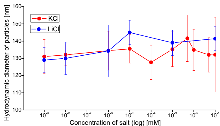
Figure 3.15. Hydrodynamic diameter of 100 nm polystyrene particles measured for different concentrations of KCl and LiCl solutions.
