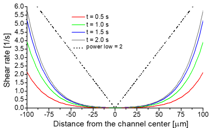
Figure 4.19. The shear rate distribution across the rectangular microchannel was calculated in a few stages of the oscillatory cycle and compared with theoretical values for parabolic flow profile (dots).
