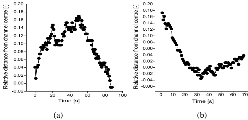
Figure 3.21. Cross-flow migration of 1 \mu\text{m} spherical particles in the oscillatory flow: (a) maximum flow velocity V_{max} = 259 \mu\text{m/s} ; Reynolds number Re = 0.063 ; relative migration velocity V_r = 7.7 \cdot 10^{-6} ; (b) V_{max} = 255 \mu\text{m/s} ; Re = 0.062 ; V_r = 2.2 \cdot 10^{-6} .
