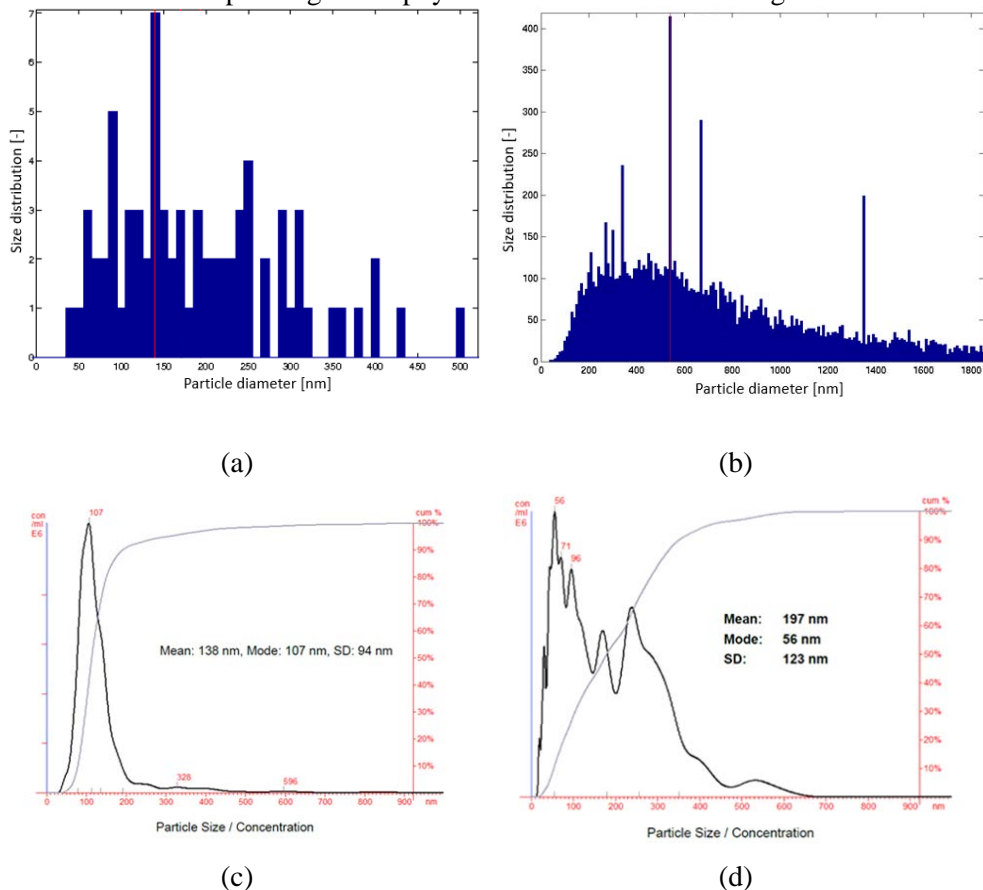
Figure 3.10. The size distribution as a function of the particle diameter: (a) 100 nm polystyrene particles suspended in 10 mM KCl solution; (b) 600 nm polystyrene particles suspended in deionized water; (c) 100 nm polystyrene particles suspended in deionized water; (d) 63 nm polystyrene particles suspended in deionized water.
