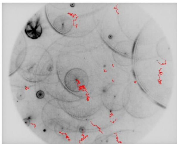
Figure 3.1. Trajectories of 100 nm gold particles dispersed in water and observed under the microscope (red tracks). Several circles indicate diffraction rings from immobile disturbances, mostly particles settled at the bottom wall.
