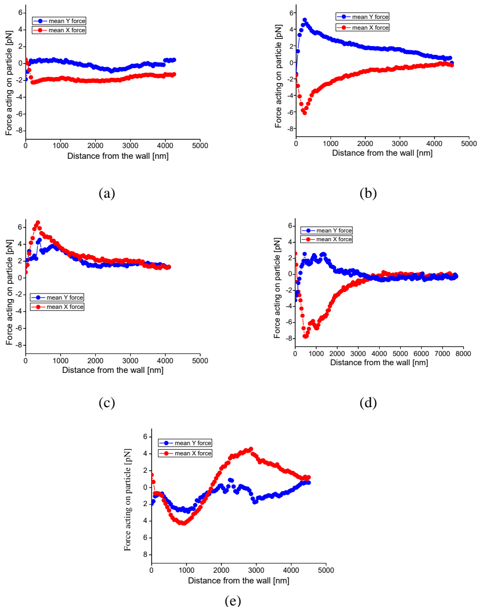
Figure 3.17. The force of the interaction between 1 \mu\text{m} polystyrene particle and PDMS wall in deionized water (a) and different KCl concentrations: (b) 0.1 mM; (c) 1 mM; (d) 10 mM; (e) 100 mM.
