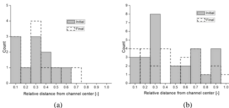
Figure 3.23. Lateral migration of spheroidal polystyrene 1 \mu\text{m} particles depending on flow rate: (a) average V_{max} = 251 \mu\text{m/s} ; (b) average V_{max} = 90 \mu\text{m/s} .
