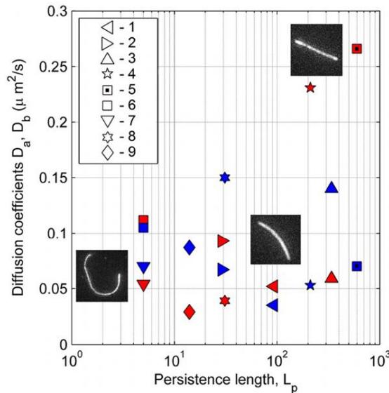
Figure 4.15. Translational diffusion coefficient D_a (red symbols) and D_b (blue symbols) as a function of persistence length for the analysed filaments shown in Table 4.2.
