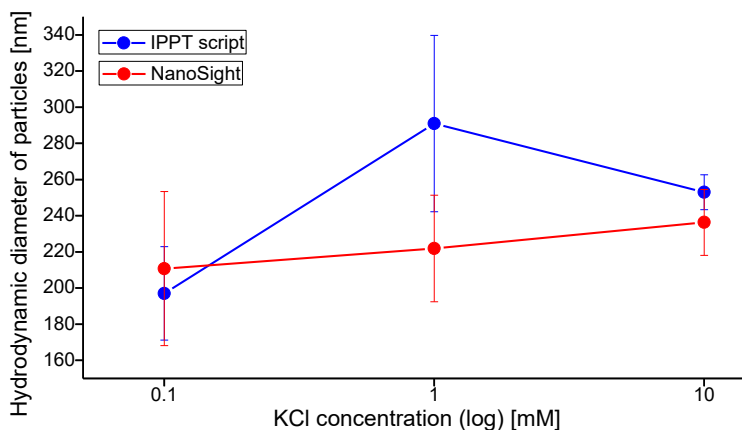
Figure 3.13. Hydrodynamic diameter of 100 nm polystyrene particles as a function of the potassium chloride concentration evaluated by IPPT script (blue dots) and a commercial NanoSight instrument (red dots).
