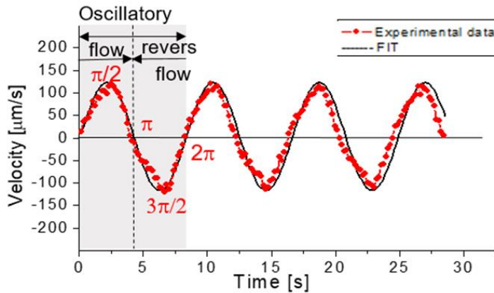
Figure 4.17. Oscillatory flow waveform generated by our home-built pulsatile pump. The horizontal solid line at V = 0 (for n\pi = 0, 1, 2 , etc.) marks cross-points of short stop-flow intervals at which some changes in nanofilament conformation and migration were recorded for each constitutive oscillatory cycle. At V = n\pi/2 (for n = 1, 3, 5 , etc.), hydrogel nanofilaments experienced the maximum flow velocity, which was used to define nondimensional flow characteristics. Empirical data are compared with the sinusoidal fit function.
