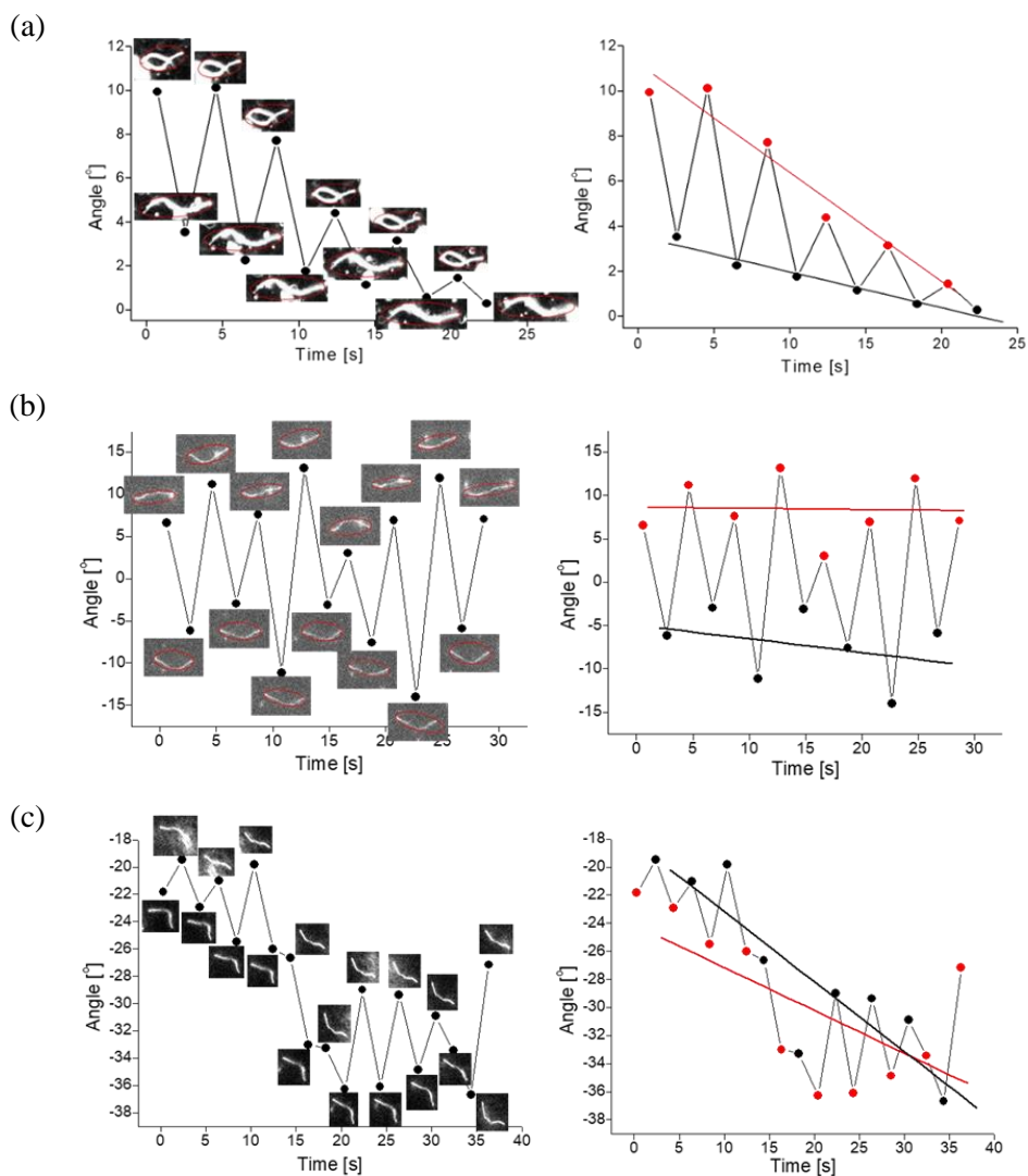
Figure 4.25. Changes in the inclination angle over time during the oscillatory flow; representative examples for bent-like (a), U-shaped buckled (b), and U-shaped stretched nanofilaments (c).
