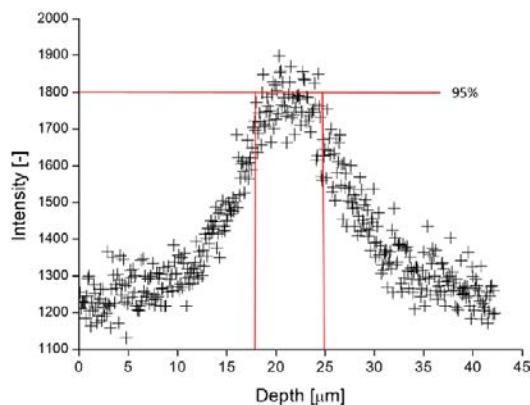
Figure 3.5. Graph indicating the focal depth of the experimental system. The intensity of the fluorescent particle was recorded for 400 steps of the microscope table moved from the top wall to the bottom wall of the channel, where the distance between steps was equal to 100 nm. The evaluated focal depth is about 10 \mu\text{m} .
