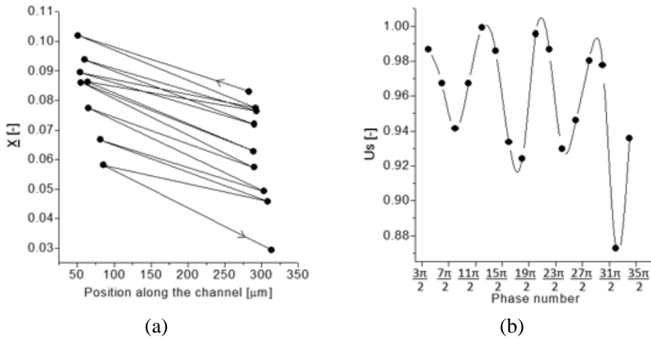
Figure 4.28. Path of the cross-flow migration of nanofilament centre-of-mass position towards the axis of the microchannel in each phase of the oscillatory flow ( n\pi , n = 1, 2, 3, \dots ); (b) Relative longitudinal slip velocity U_s of the nanofilament during each oscillating flow maximum ( n\pi/2 , n = 1, 3, 5, \dots ).
