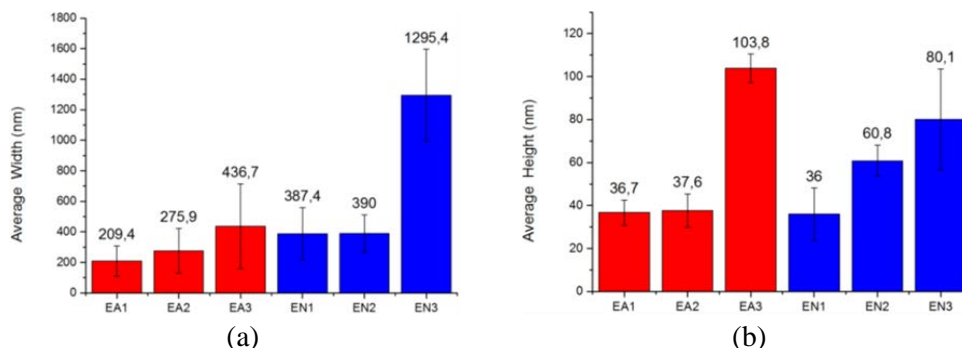
Figure 4.10. Average width (a) and height (b) of the analysed hydrogel nanofilaments.
