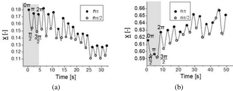
Figure 4.29. Trajectories of the centre-of-mass position of nanofilaments in the function of time: (a) towards the channel centre ( d = 105 \text{ nm} , L = 41 \text{ }\mu\text{m} , V_{max} = 250 \text{ }\mu\text{m/s} , U_r = 0.85 \cdot 10^{-3} ); (b) towards the wall ( d = 134 \text{ nm} , L = 54 \text{ }\mu\text{m} , V_{max} = 132 \text{ }\mu\text{m/s} , U_r = 0.6 \cdot 10^{-3} ).
