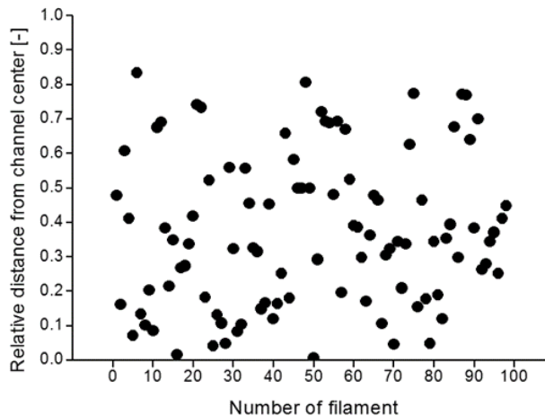
Figure 4.27. Initial distribution of 100 experimental sequences of investigated nanofilaments across the whole plane of the microchannel.
