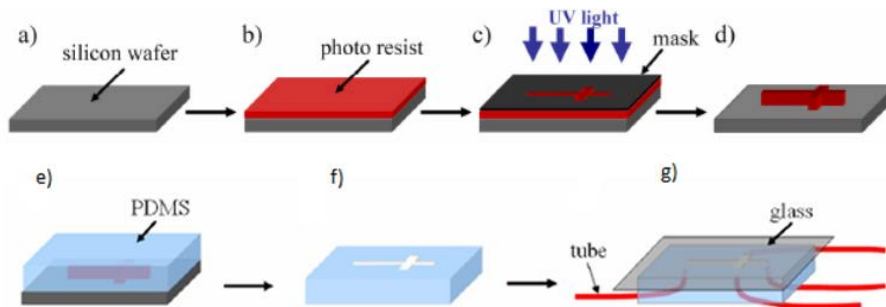
Figure 2.3. Photolithography and fabrication of a PDMS microfluidic system [26].
