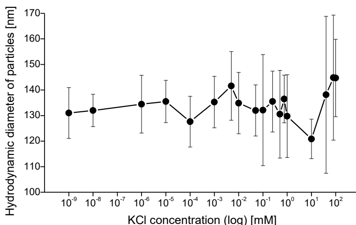
Figure 3.11. Hydrodynamic diameter of 100 nm polystyrene particles obtained at different concentrations of KCl.
