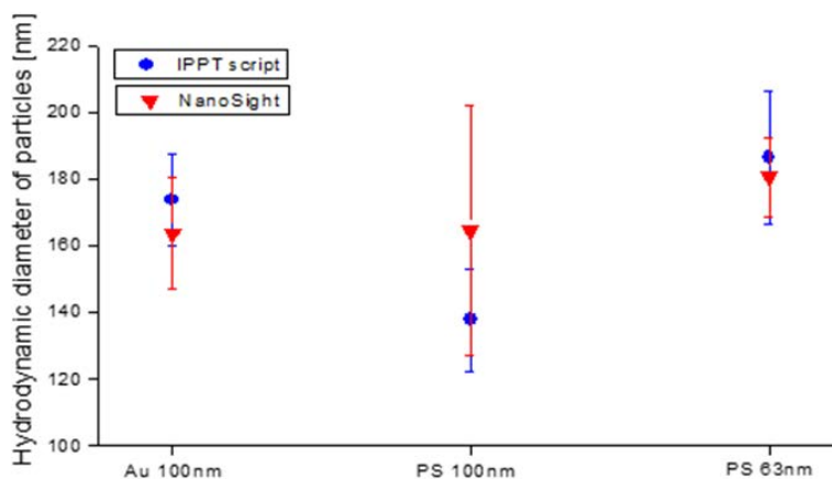
Figure 3.9. Comparison of hydrodynamic diameter results obtained for three particle types: Au100nm – 100 nm gold particles, PS100nm – 100 nm polystyrene particles, PS63nm – 63 nm polystyrene particles. Experiments performed in deionized water. Red dots – Nanosight results, blue dots – IPPT particle tracking scrip.
