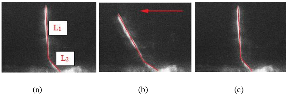
Figure 4.16. Bending of a filament in a flow recorded by fluorescence microscopy; (a) – initial position, (b) – bending of the filament triggered by the flow, (c) – returning phase of the filament after the flow was stopped. L_1 – stiff part of the filament, L_2 – flexible part of the filament attached to the wall.
