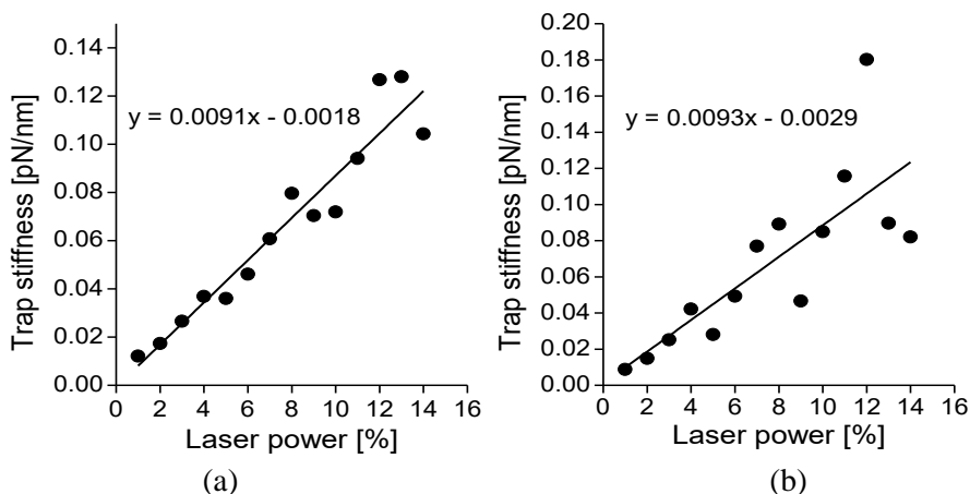
Figure 3.16. The stiffness of the optical trap in X (a) and Y (b) direction as a function of the trapping laser power.
