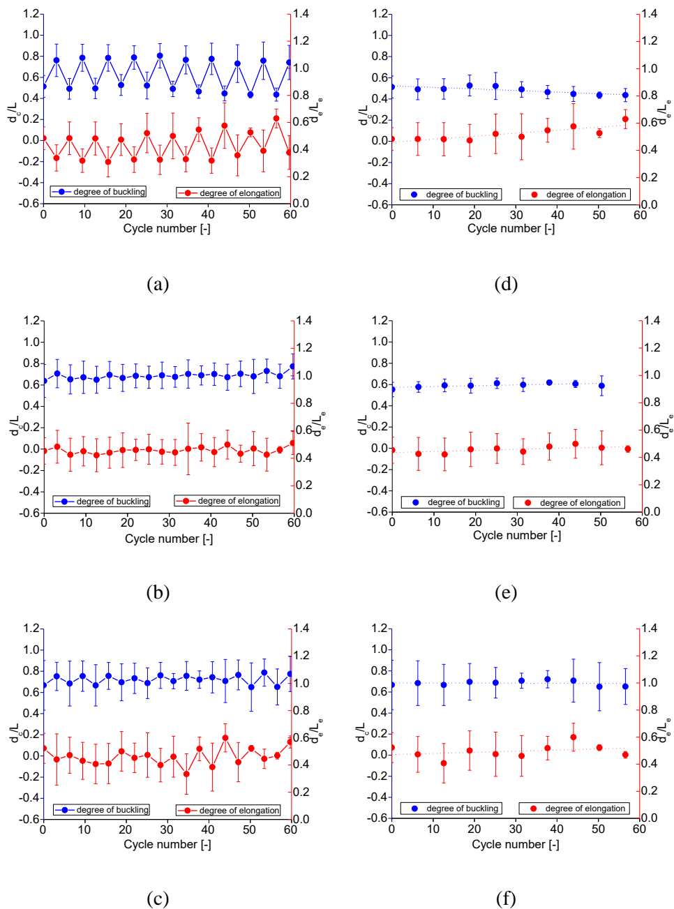
Figure 4.22. Changes in the degree of buckling and elongation parameters for (a) bent-like filaments, (b) U-shaped stretched filaments, (c) U-shaped buckled filaments in each phase; (d, e, f) – in 2\pi phase. Left axis – BU, right axis – EL.
