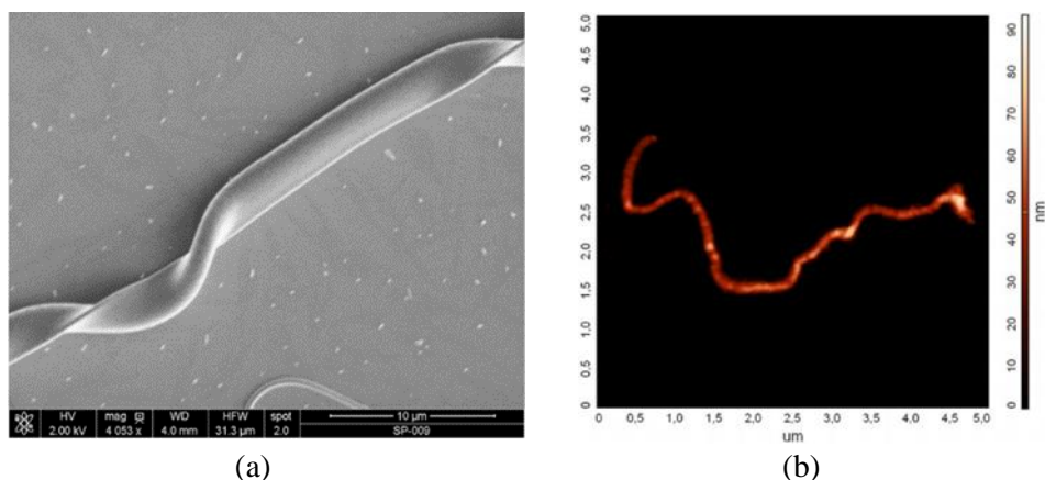
Figure 4.9. (a) Micrograph of a ribbon-like core-shell PLCL/PAAm nanofibre (EA3) observed under SEM; (b) Topography of a ribbon-like nanofilament (EA1) observed by AFM (width 128 nm, contour length 7 μm, height 39 nm, equivalent diameter 80 nm).
