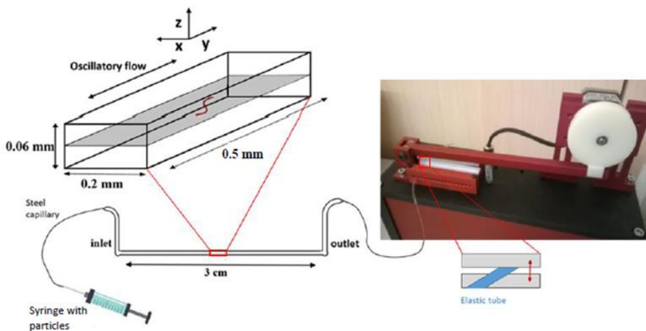
Figure 3.4. Experimental set up for the analysis of nanoobject dynamics. The experimental channel and pulsatile pump were connected with the reservoir (syringe) by a steel capillary.
