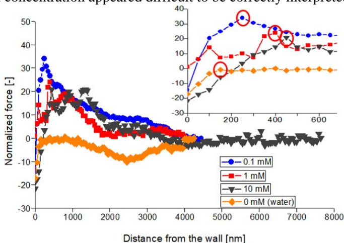
Figure 3.18. The force of the interaction between 1 \mu\text{m} polystyrene particle and PDMS wall in deionized water and in different KCl concentration.
