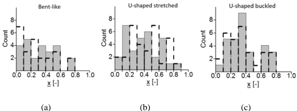
Figure 4.31. The centre-of-mass distribution of hydrogel nanofilaments across the microchannel width \underline{x} (0 and 1 denote the microchannel centreline and wall, respectively), before the application of the oscillating hydrodynamic force (grey bars), and after over 40 oscillatory cycles (dashed-contour bars).
