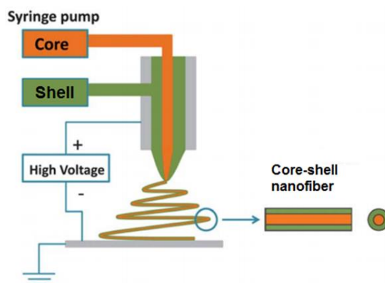
Figure 2.1. Coaxial electrospinning setup for core-shell fibres [38].
