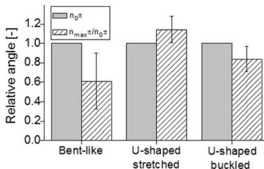
Figure 4.26. Relative changes of the filament inclination angle after applying a flow: initial status ( grey bars ) and after the final oscillatory cycle ( dashed-patterned bars ). Data are normalized to the initial inclination angle.
