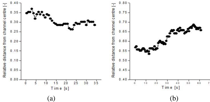
Figure 3.22. Cross-flow migration of 1 \mu\text{m} spherical particles in the oscillatory flow: (a) maximum flow velocity V_{max} = 252 \mu\text{m/s} ; Reynolds number Re = 0.061 ; relative migration velocity V_r = 7.2 \cdot 10^{-6} ; (b) V_{max} = 228 \mu\text{m/s} ; Re = 0.060 ; V_r = 6.5 \cdot 10^{-6} .
