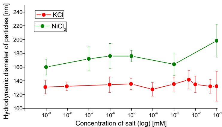
Figure 3.12. Hydrodynamic diameter of 100 nm polystyrene particles obtained at different concentrations of monovalent (KCl) and divalent (NiCl 2 ) solutions.
