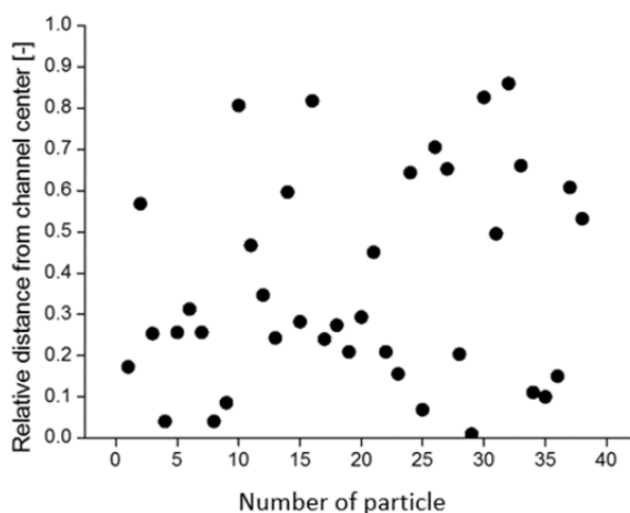
Figure 3.20. Initial position of each examined particle in the microchannel; the relative distance [0,1] denotes the microchannel centre and the wall, respectively.
