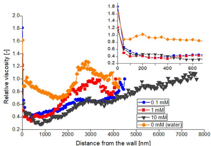
Figure 3.19. The effective viscosity as a function of distance between wall and approaching to it particle, for water and different concentrations of salt.
