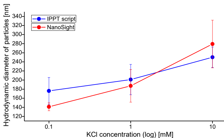
Figure 3.14. Hydrodynamic diameter of 63 nm polystyrene particles as a function of the potassium chloride concentration evaluated by IPPT script and the commercial NanoSight instrument.
