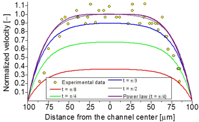
Figure 4.18. Velocity flow field from finite element method simulations of the oscillatory flow. Yellow dots represent experimental data; the violet line signifies fit by higher order parabola; red, green, blue, and grey lines represent the results of numerical simulations obtained for different time steps.
