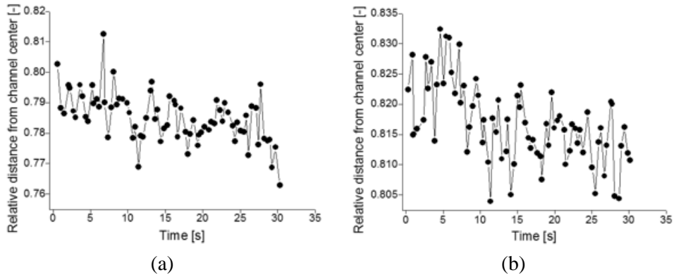
Figure 4.30. Lateral migration of nanofilaments conveyed by the oscillating flow, observed close to the microchannel wall. Dots indicate the position of the centre of mass recorded at zero flow velocity ( n\pi/2 ), (a) d = 125 \text{ nm} , L = 27 \text{ }\mu\text{m} , V_{max} = 83 \text{ }\mu\text{m/s} , U_r = 1.34 \cdot 10^{-3} ; (b) d = 114 \text{ nm} , L = 30 \text{ }\mu\text{m} , V_{max} = 75 \text{ }\mu\text{m/s} , U_r = 0.4 \cdot 10^{-3} .
