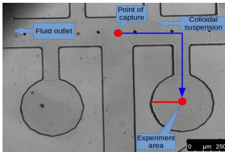
Figure 3.2. Microchannels with round wells designed for experiments with optically trapped particles. Circle chambers had a diameter of 200 \mu\text{m} and depth of 60 \mu\text{m} . The red arrow indicates the direction in which the wall moves as a result of the microscopic table moving [52].
