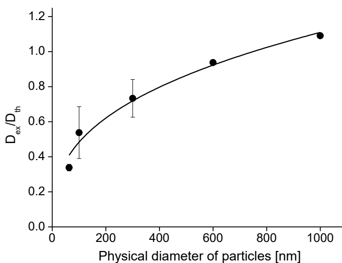
Figure 3.8. Dependence of the relative diffusion coefficient (ratio of experimental to theoretical diffusion coefficients) on the physical diameter for polystyrene particles suspended in deionized water.
