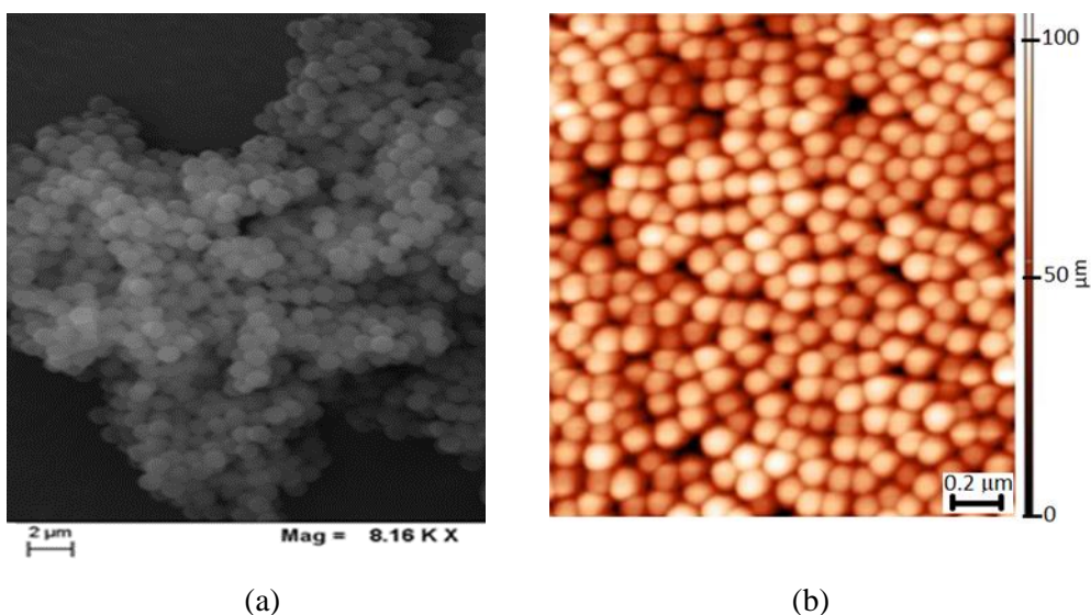
Figure 3.6. (a) 1 μm polystyrene particles observed by SEM; (b) AFM image of 100 nm polystyrene particles, substrate: silicon.
