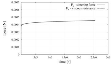
Figure 5.4. Evolution of sintering force and viscous resistance at free sintering of two particles of Cu – mass scaling factor 10^{14} .
