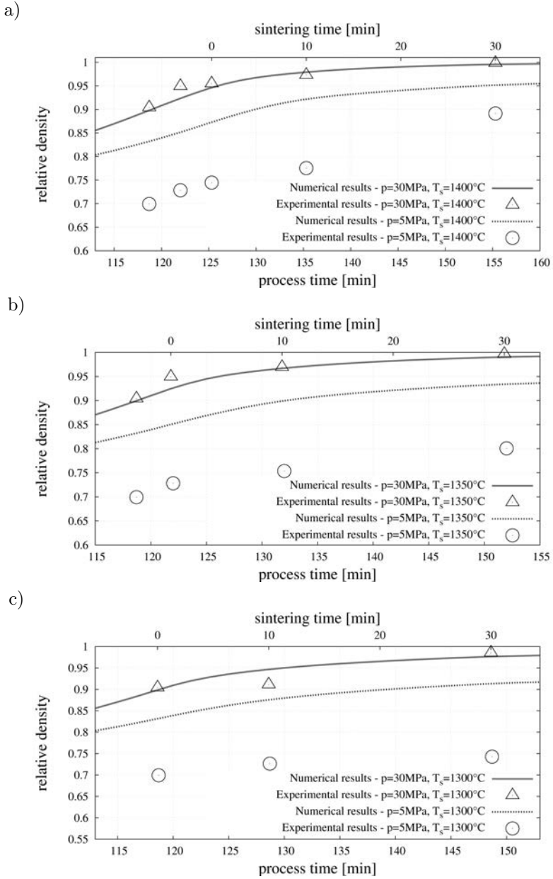
Figure 5.41. Density evolution – numerical and experimental results of composite NiAl-Al 2 O 3 powder sintering for pressure 5 and 30 MPa and sintering temperature of: a) T_s = 1400^\circ\text{C} , b) T_s = 1350^\circ\text{C} , c) T_s = 1300^\circ\text{C} .
