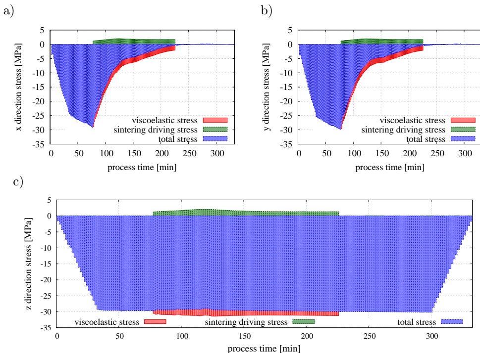
Figure 6.7. Evolution of the total, sintering and viscoelastic macroscopic stress: a) in x direction, b) in y direction, c) in z direction.
