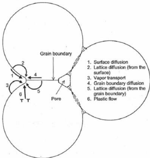
Figure 2.2. Material transport pathways to the neck area [3].
