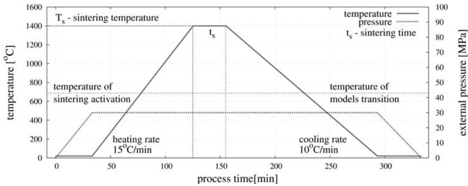
Figure 5.22. Temperature and pressure profiles for the powder metallurgy process of intermetallic powder at T_s = 1400^\circ\text{C} , t_s = 30 min and p = 30 MPa.
