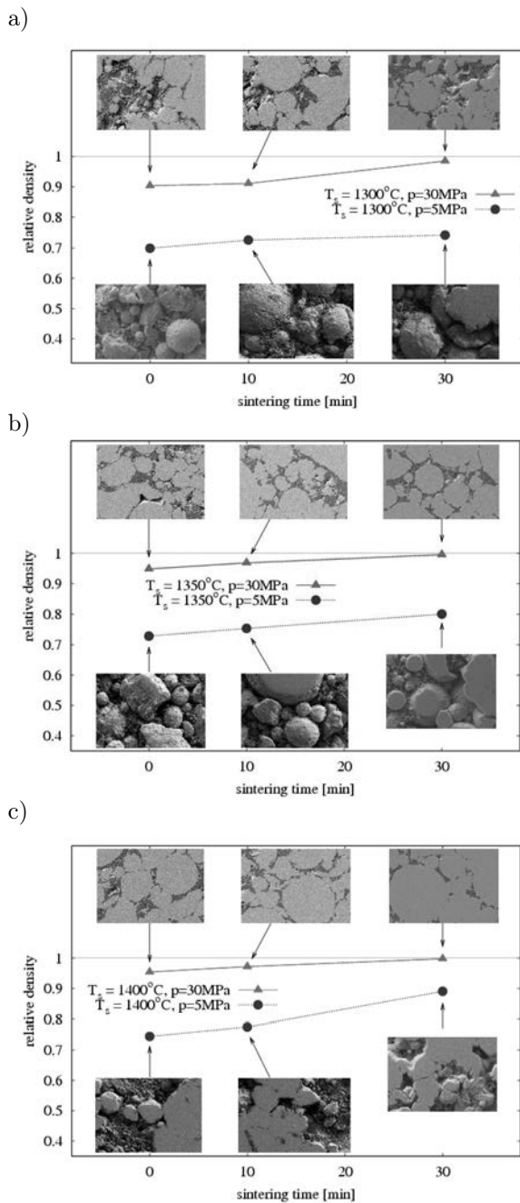
Figure 3.11. Density evolution results of NiAl/ \text{Al}_2\text{O}_3 composite sintering with pressure 5 and 30 MPa at sintering temperature of: a) T_s = 1300^\circ\text{C} , b) T_s = 1350^\circ\text{C} , c) T_s = 1400^\circ\text{C} .
