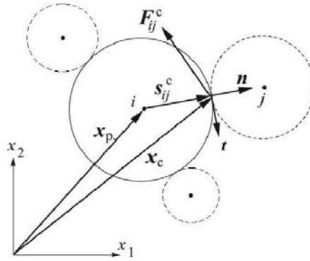
Figure 6.3. Definition of inter-particle interaction [226].
