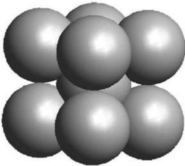
Figure 5.7. BCC sphere packing.
