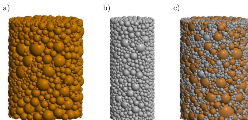
Figure 5.17. Discrete element specimens of a) one-phase NiAl powder, b) one-phase Al 2 O 3 powder, c) two-phase 80%NiAl-20%Al 2 O 3 powder.
