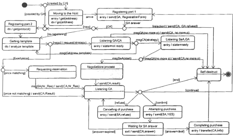
Fig. 4. Buyer Agent Statechart diagram
