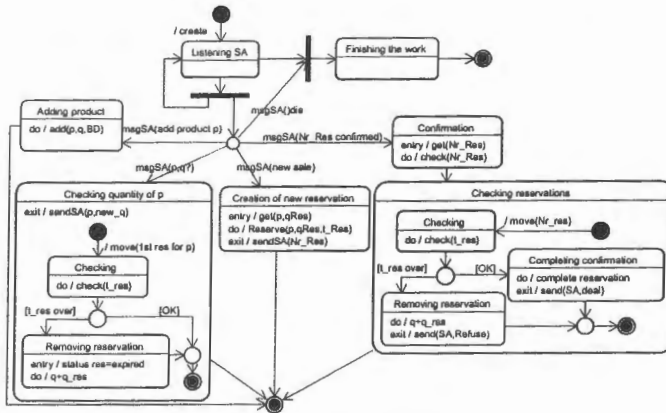
Fig. 8. Warehouse Agent Statechart diagram
