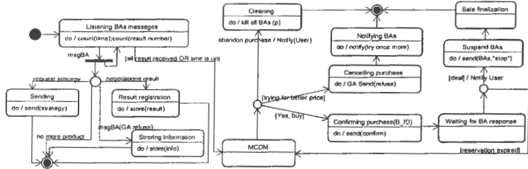
Fig. 3. Client Agent Statechart diagram
