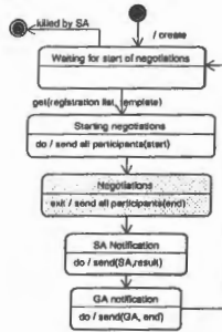
Fig. 9. Seller Agent Statechart diagram
