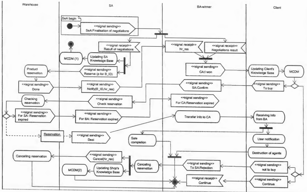
Fig. 11. Activity Diagram—after negotiation process
