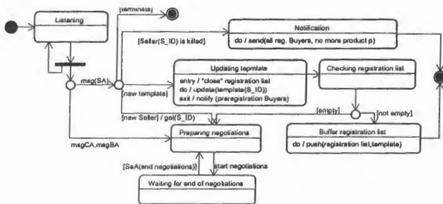
Fig. 6. Gatekeeper Agent Statechart diagram
