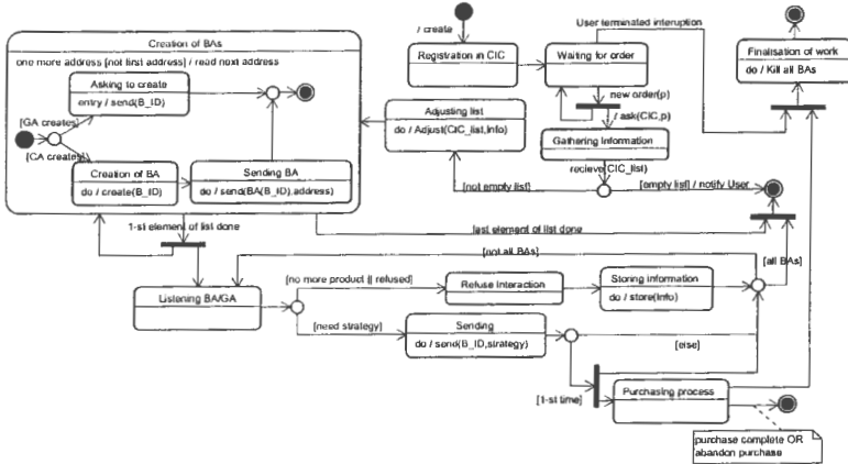
Fig. 2. Client Agent Statechart diagram
