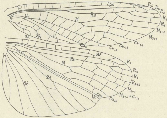
Fig. 3.—Venation of Tasmanoperla diversipes n. g. et. sp.; family Austroperlidæ.
