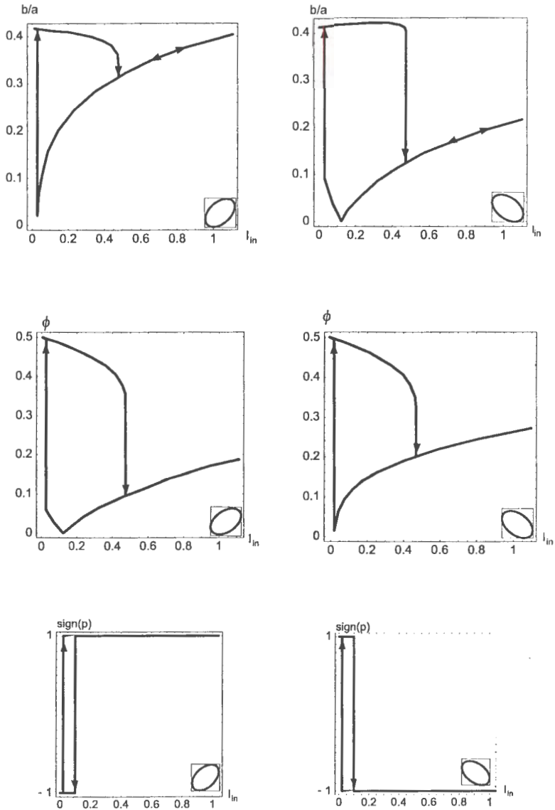
Fig.2 Comparison of polarisation state parameters of the outgoing wave as function of the intensity of the incident wave with elliptic polarisation (two cases are shown on inserts in the right bottom corners. Left column corresponds to \delta = \pi/4 , the right one to \delta = -\pi/4 )
