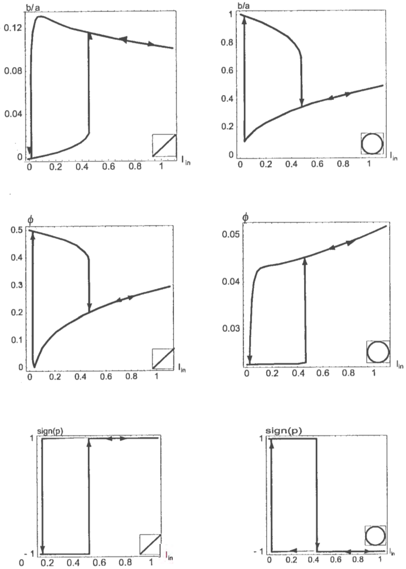
Fig. 1 Polarisation state parameters of the outgoing wave as functions of incident wave intensity I_{in} (in arbitrary units) for two different polarisations of the incident wave: linear (left part, \delta = 0 ) and circular (right part, \delta = \pi/2 ).
