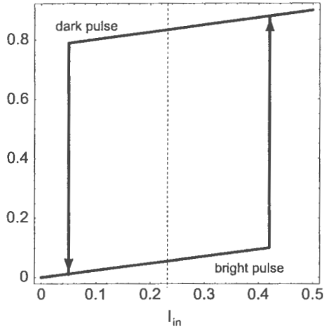
Fig. 3 The principle of switching between optical states of an optical logic gate. The digit "1" represents the dark pulse, whereas "0" – the bright pulse
